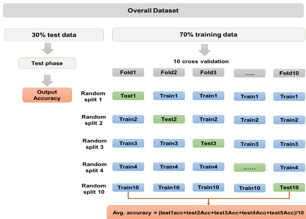
Fig. 2. k-fold cross validation different feature sets, tweaking algorithm settings, orchanging which genetic markers are used.
