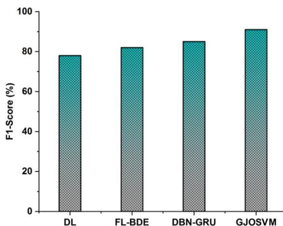
Fig. 6. F1-Score
