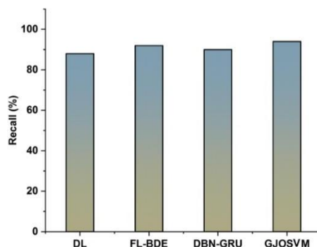
Fig. 5. Recall
