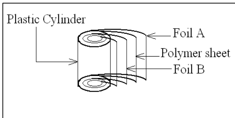
Figure 4: Design of a capacitive sensor.
