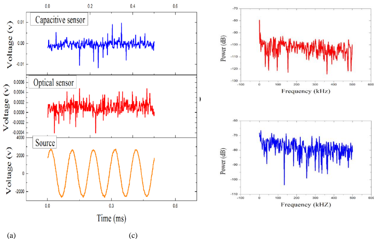
Figure 7: (a) The signal (in time domain) captured by CS and FOS together with the high voltage probe signal at 5.5 kV p-p. The signal after FFT of (b) FOS and (c) CS.
