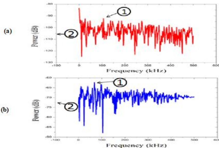
Figure 11: The FFT spectra of the output corresponding to 28 kV p-p probe signal for (a) FOS and (b) CS.
