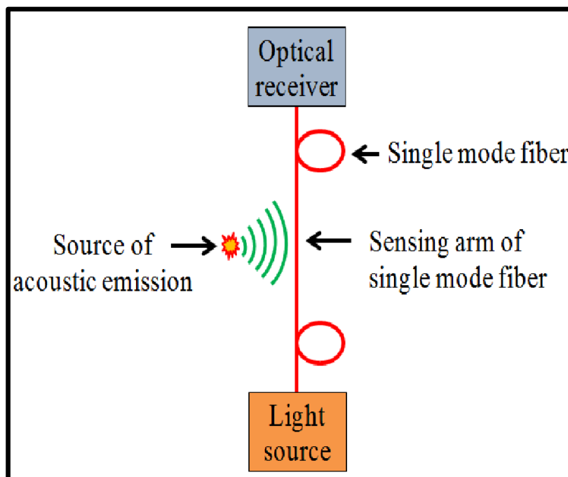
Figure 3: Schematic for AE detection.
