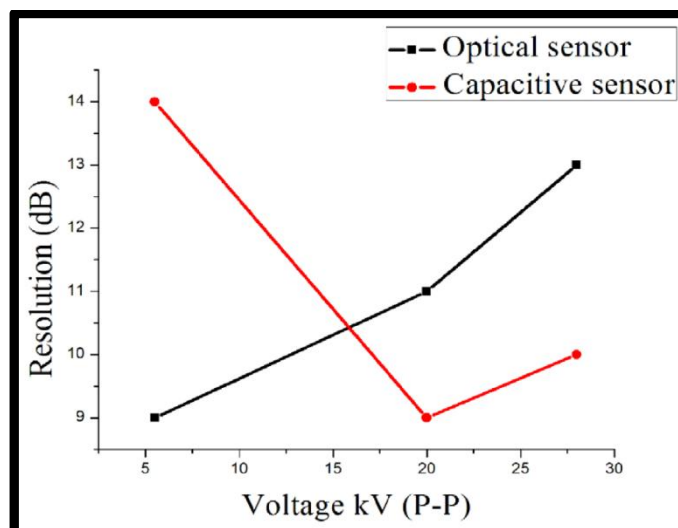
Figure 12: Resolution characteristics of FOS and CS.
