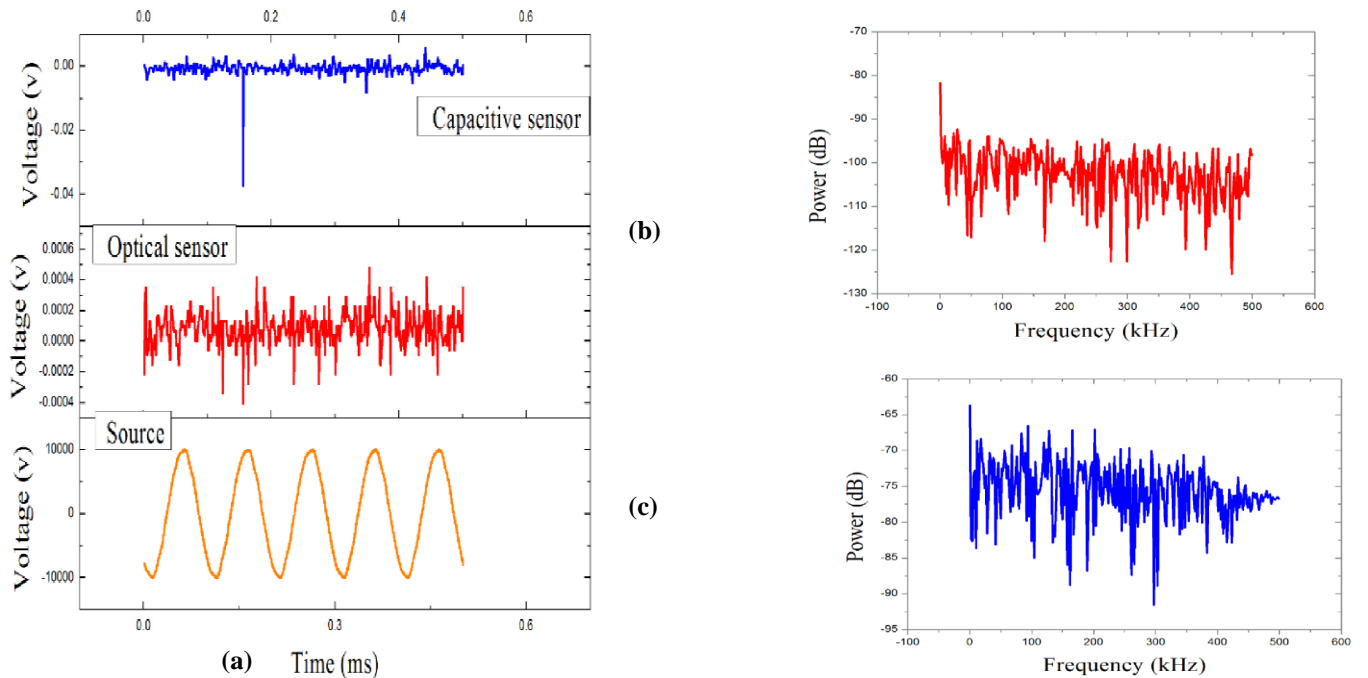
Figure 8: (a) The signal (in time domain) captured by CS and FOS together with the high voltage probe signal at 20 kV p-p. The signal after FFT of (b) FOS and (c) CS.
