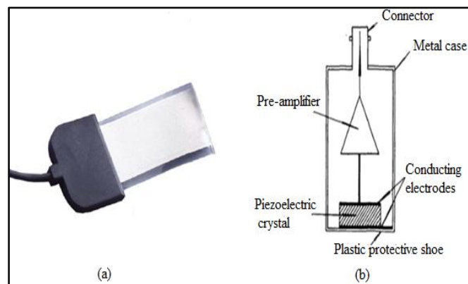
Figure 2: Piezoelectric transducer sensor: (a) film sensor with connectors and (b) typical design [8].
