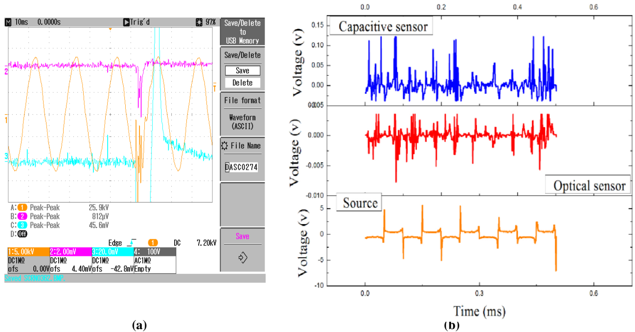
Figure 10: Patterns for three signals at break down voltage (a) from oscilloscope and (b) in time domain.
