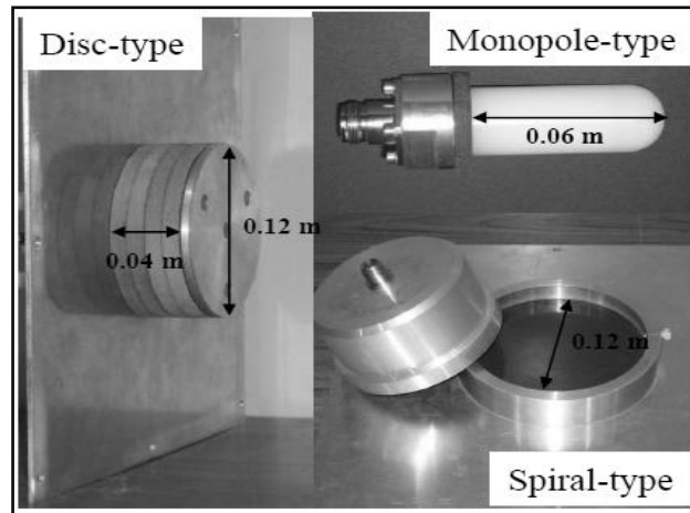
Figure 1: Disc, monopole and spiral -type UHF sensors [10].
