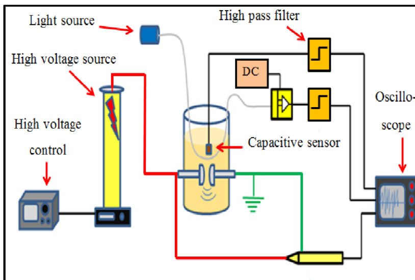
Figure 6: Schematics showing working principle of the detection using two sensors.
