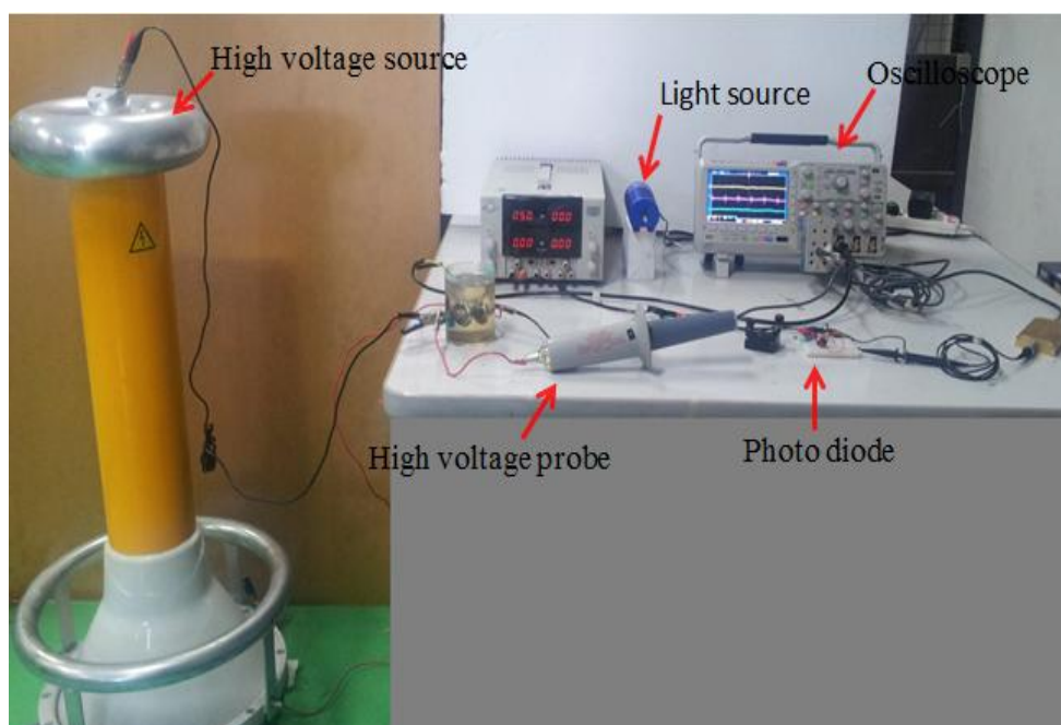
Figure 5: Experimental set up for PD signal detection in the insulation oil using FOS and CS.
