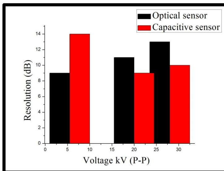
Figure 13: Levels of resolution for FOS and CS.
